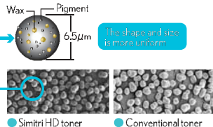
Comparison of conventional toner and Simitri HD toner. (Internal testing)
